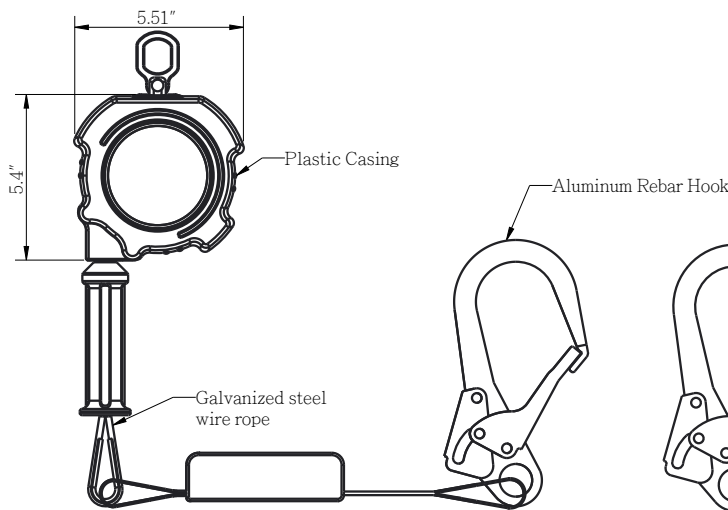
FRONT VIEW SRL1411242
